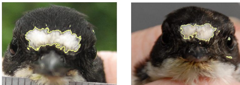
Figure 11: Blaze segmentation
