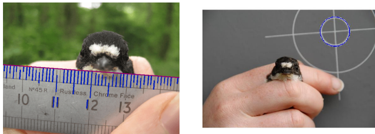
Figure 15: Hough transform used for detecting geometrical objects. Left: lines detection using MATLAB routines houghlines , houghpeaks . Right: circle detection using MATLAB routine imfindcircles .
