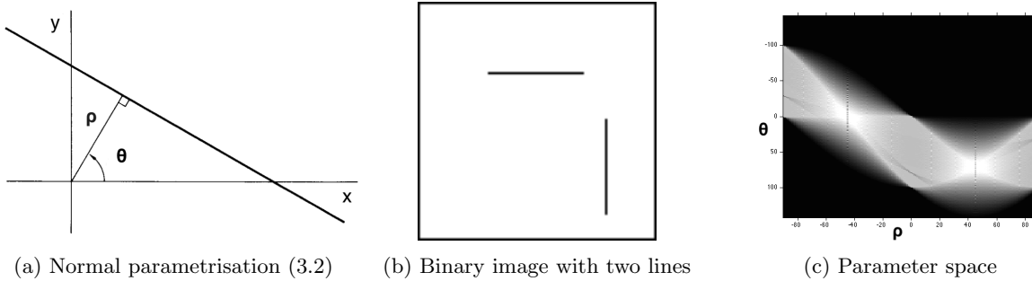
Figure 5: Normal form: image and parameter spaces.
